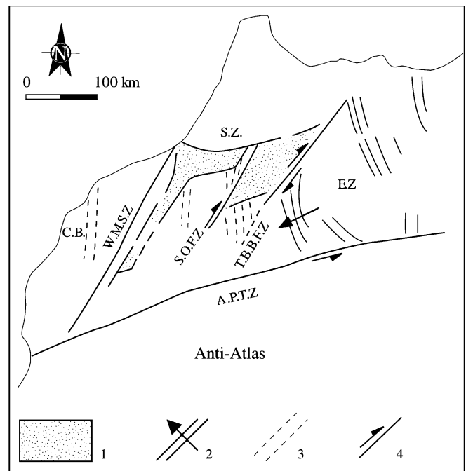
Fig. 7. Opening model of the Carboniferous basins (from Bouabdelli and Piqué, 1996). 1: Sidi-Bettache and Azrou-Khenifra basins. 2: Eovariscan structures and vergence (eastern zone—EZ). 3: Suspected eovariscan structures in the anticline zones. 4: Strike-slip along the main faults. CB: Coastal Block; SZ: Sehoul Zone.
