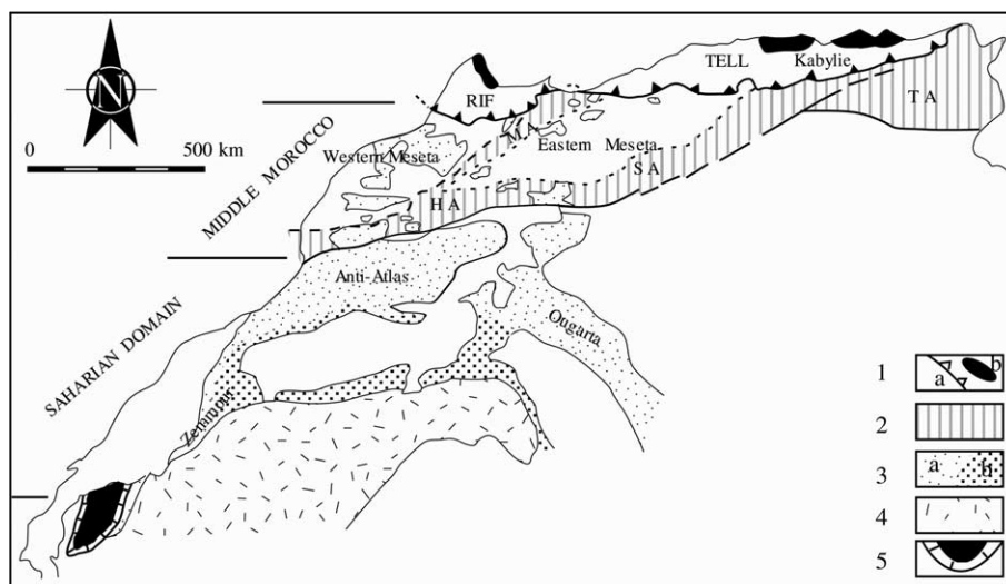
Fig. 1. Structural subdivisions of North Africa and location of the Paleozoic terranes. 1: Rifian-Tellian belt, a: southern front of the chain; b: Paleozoic allochthonous terranes of the internal zones. 2: Atlasic belt (HA: High Atlas, SA: Saharian Atlas, TA: Tunisian Atlas, MA: Middle Atlas). 3: Paleozoic, a: deformed by variscan orogeny, b: undeformed. 4: West African craton (Archean and Proterozoic massifs). 5: Mauritanides allochthonous.
