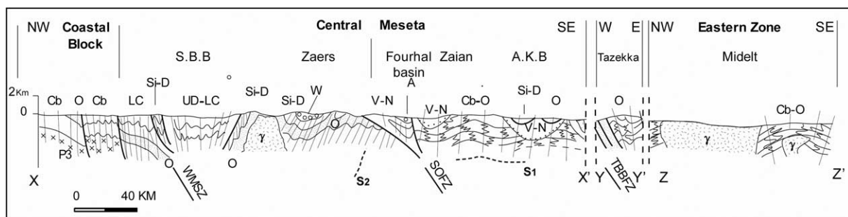
Fig. 5. Simplified geological section across the northern mesetian domain (see location on the Fig. 2). P3: Neoproterozoic; Cb: Cambrian; O: Ordovician; Si–D: Silurian to Middle Devonian; UD–LC: Upper Devonian, Lower Carboniferous; V–N: Viséan–Namurian; W: Upper Westphalian; A: Autunian; \gamma : granitoids. S1: eovariscan cleavage, S2: main variscan cleavage. SBB: Sidi-Bettache Basin, AKB: Azrou-Khénifra Basin.
