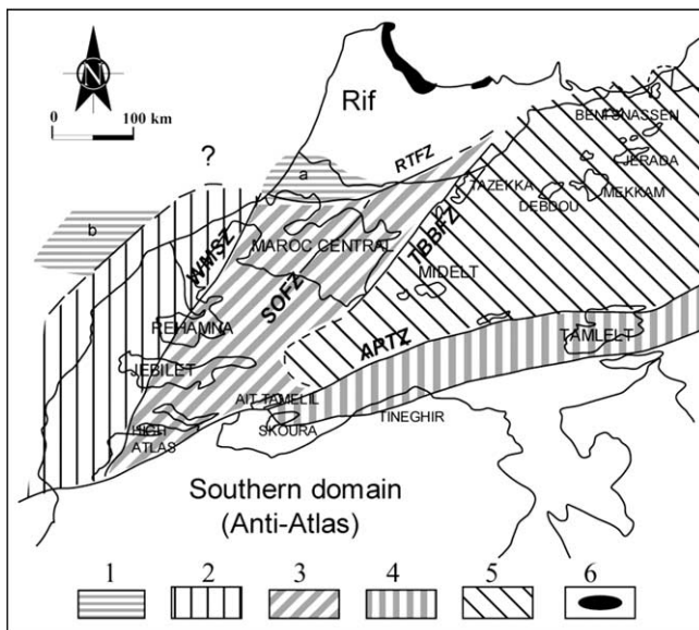
Fig. 4. The main structural zones of the northern domain (Meseta s.l. ) with the most important variscan inliers. 1: Sehoul Zone (a) and its likely prolongation to the west (b) with “Caledonian” events. 2: Coastal Block: lower and middle Paleozoic, weakly deformed. 3: Central Meseta: lower to upper Paleozoic with carboniferous pull-apart and foreland basins, strongly deformed by variscan phases. 4: Southern Zone: lower to upper Paleozoic similar to the southern domain (Anti-Atlas), moderately folded by the variscan phases. 5: Eastern Zone: lower and middle Paleozoic deformed by eovariscan events, small carboniferous basins with calc-alkaline volcanism. 6: Internal zones of the Rifian chain. Main structural limits: RTFZ: Rabat-Tiflet Fault Zone, WMSZ: Western Meseta Shear Zone, SOFZ: Smaala-Oulmès Fault Zone, TBBFZ: Tazekka-Bsabis-Bekrit Fault Zone, APTZ: Atlas Paleozoic Transform Zone.
