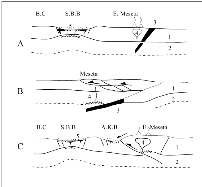
Fig. 8. Geodynamical models for the Moroccan Hercynides (Middle Carboniferous). Subducted oceanic crust: A from Kharbouch et al. (1985); B from Roddaz et al. (2002). Intracontinental shear zones, C from Kharbouch (1994); and Piqué (2001). 1: continental crust; 2: upper mantle; 3: oceanic crust; 4: calc-alkaline magmatism; 5: alkaline to tholeiitic magmatism. CB: Coastal Block; SBB: Sidi Bettache Basin; AKB: Azrou Khenifra Basin.
