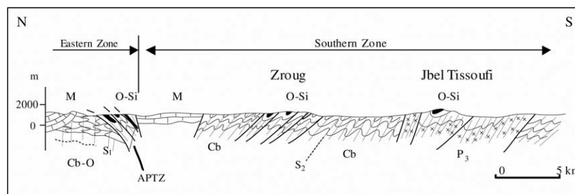
Fig. 6. Simplified geological section across the Tamlelt inlier (from Houari and Hoepffner, 2000; location on Fig. 2). P3: Neoproterozoic, Cb: Cambrian; O-Si: Ordovician and Silurian; Cb-O: Cambrian-Ordovician (eastern zone); M: mesozoic cover (High Atlas). S1: covariscan cleavage, S2: main variscan cleavage.
