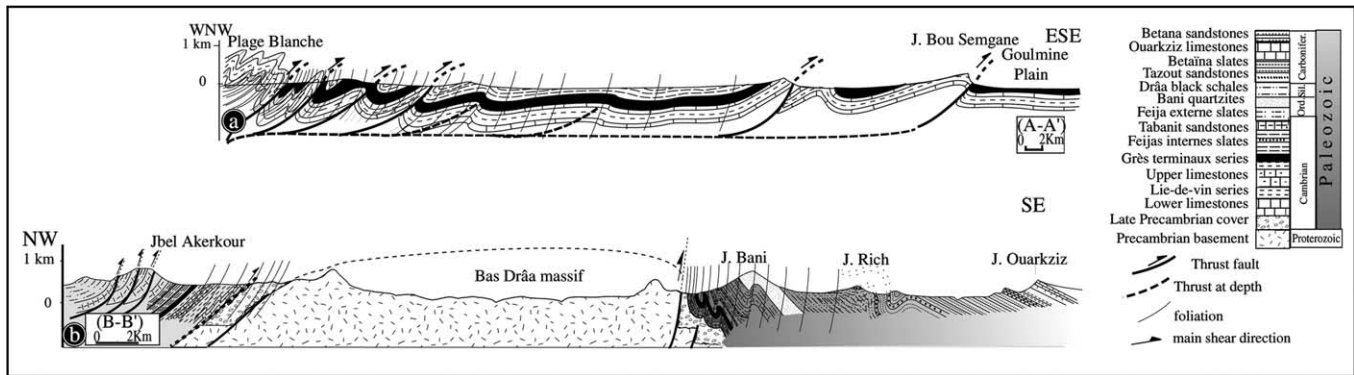
Fig. 3. Geological sections across the north western part of the Anti Atlas domain (see location on Fig. 2).
