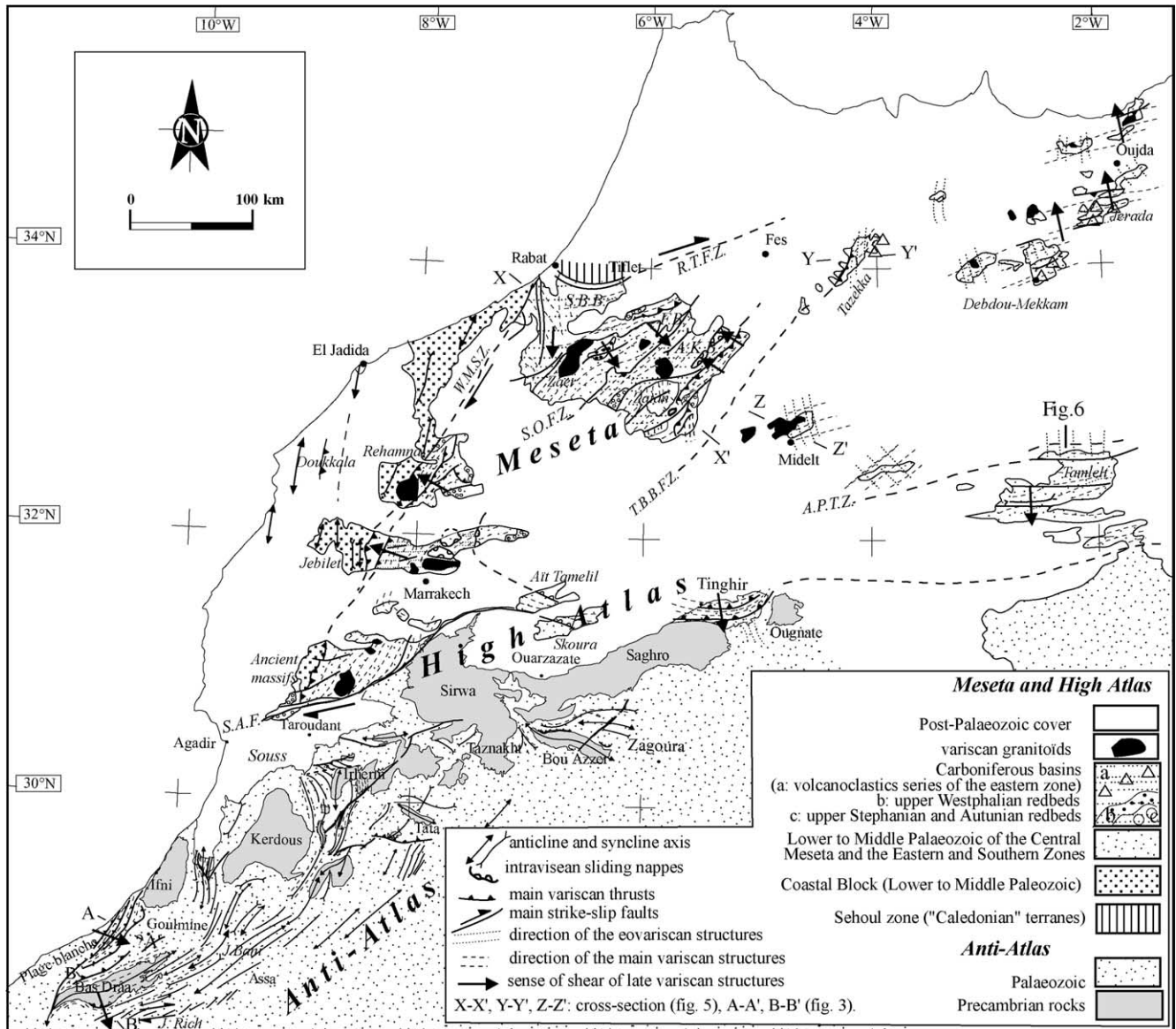
Fig. 2. Structural map of the northern (Meseta) and southern (Anti Atlas) domains.
