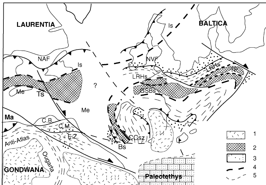
Fig. 9. Possible configuration of the periatlantic paleozoic orogens in Permian time (from Matte, 2001; Houari and Hoepffner, 2003). 1: Gondwanan stable blocks (West African Shield); 2: Parts of Avalonia and Armorica microplates; 3: Carboniferous foreland basins; 4: main sutures (Is: Iapetus suture; Ts: Theic suture; Bs: Beja suture; CCsz: Coimbra-Cordoba shear zone; LRHs: Lizard Rheno-Hercynian suture; TP: Tepla suture; GSBs: Galicia South-Brittany suture). NAF: North Appalachian Front; NVF: North Variscan Front; Me: Meguma Zone and *: Caledonian terranes (like Schoul Zone); CB: Coastal Block; CM: Central Meseta; EZ: Eastern Zone; AA: Anti-Atlas; Ma: Mauritanides belt.
